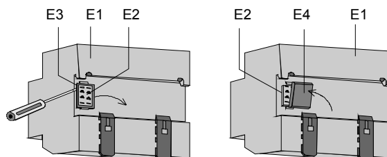
Figure 4: Covering the contact system
